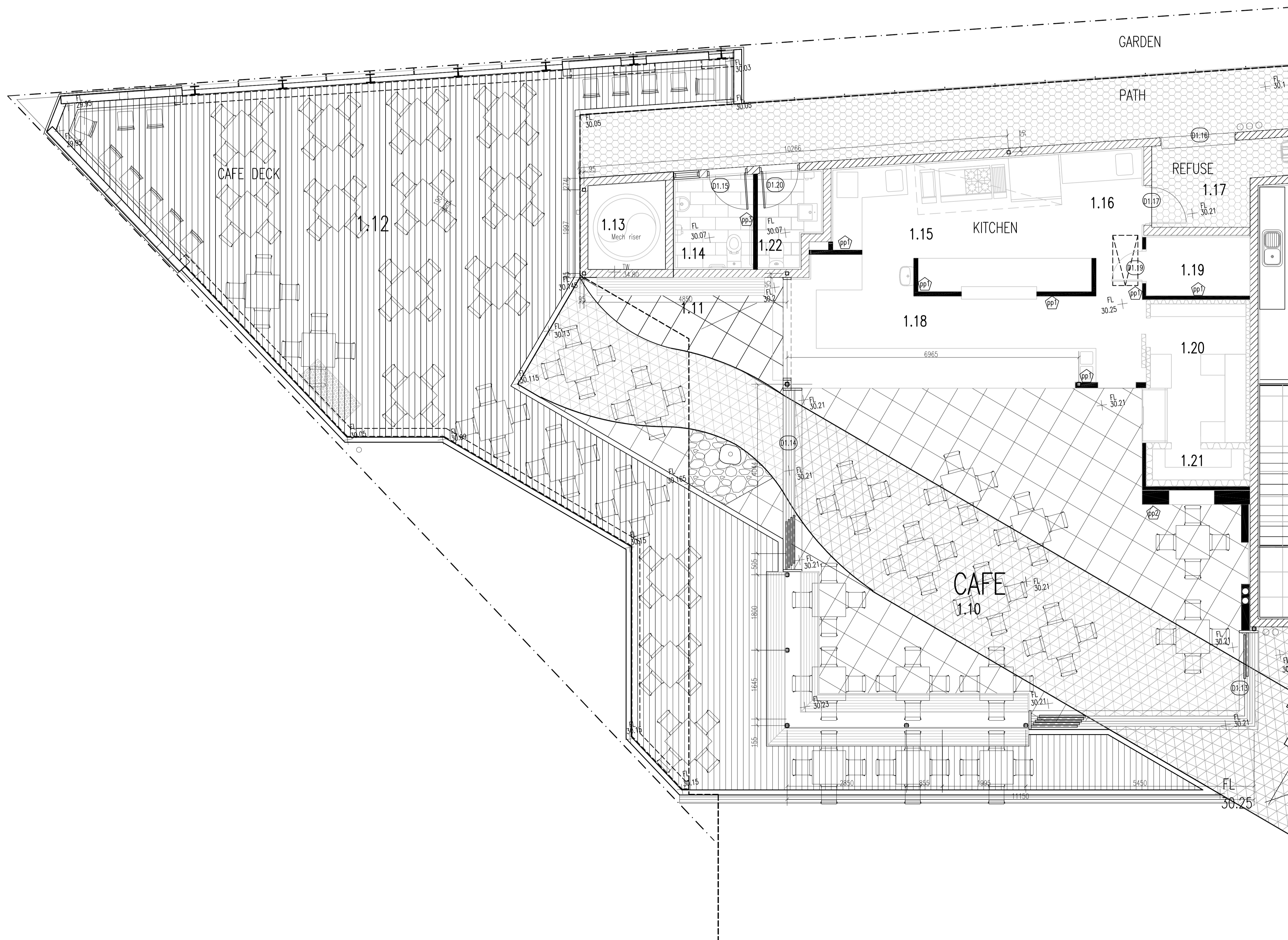
CAFE FLOOR PLAN
